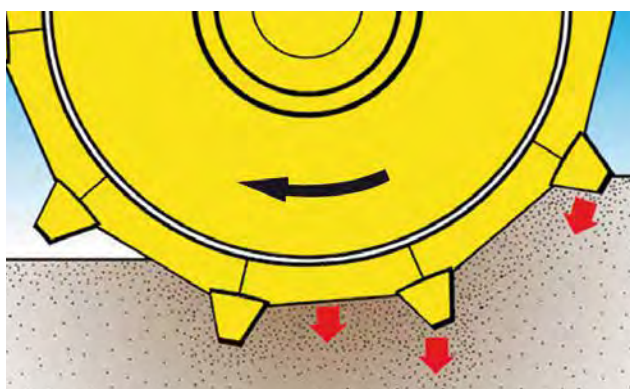
Polygon disc wheels with compressor teeth for crushing, kneading and effective compaction at depth.
