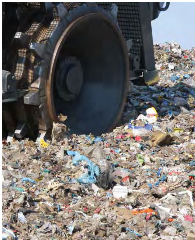
Scrapers ensure clean wheels and high compaction.
