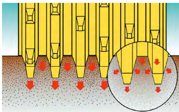
Additional lateral forces increase compaction.
